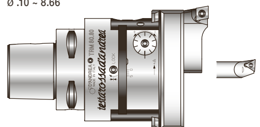
PSC63 - TRM80 INCH \varnothing .10 ~ 8.66
