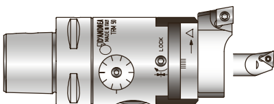
PSC50 - TRM50 INCH \varnothing .10 ~ 5.51
