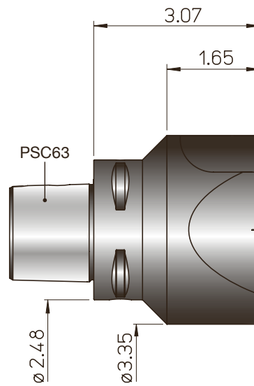
PSC63 - TS63 \varnothing 3.54 ~ 4.72
