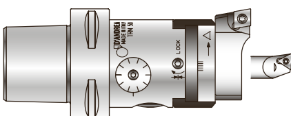
PSC63 - TRM50 INCH \varnothing .10 ~ 5.51
