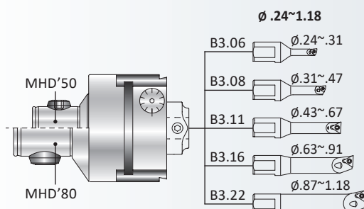
KIT K01 TRM 50/80 - 80/80
